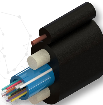
Toneable Flat Drop Cables
